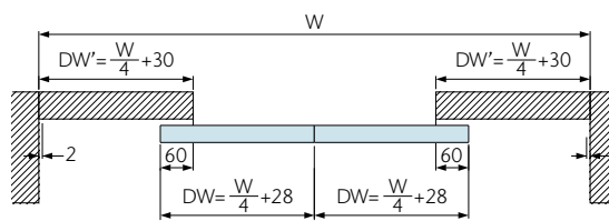
Glas/Glass/Verre double system
